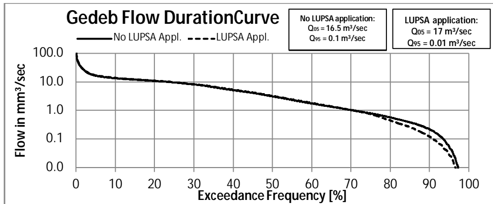
Figure 4: LUPSA application lead impact on the flow duration curve
