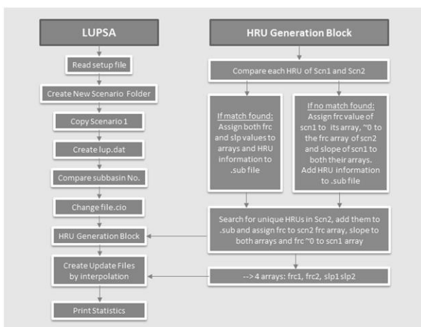
Figure 3: LUPSA workflow (Scn = Scenario, lup.dat = SWAT land use update file, frc = fraction, slp = slope)
