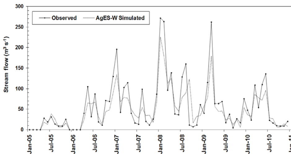
Figure 2. Average monthly Upper CCW streamflow ( m^3 s^{-1} ) at gauge F34 (January 2005 to December 2010).
