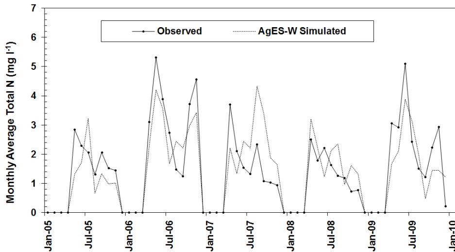
Figure 3. Average monthly Upper CCW total N ( \text{mg l}^{-1} ) at gauge F34 (May 2005 to December 2009).
