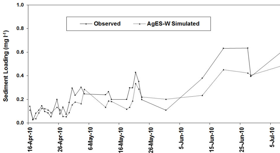
Figure 4. Daily Upper CCW sediment loading ( \text{mg l}^{-1} ) at gauge F34 (April 2010 to July 2010).
