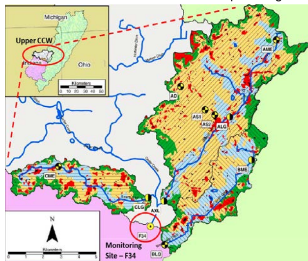
Figure 1. Upper CCW stream network and gauging stations.
