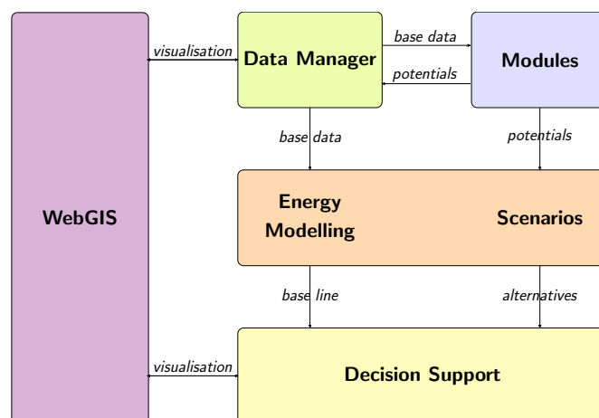
Figure 1: The iGUESS user interface components.
