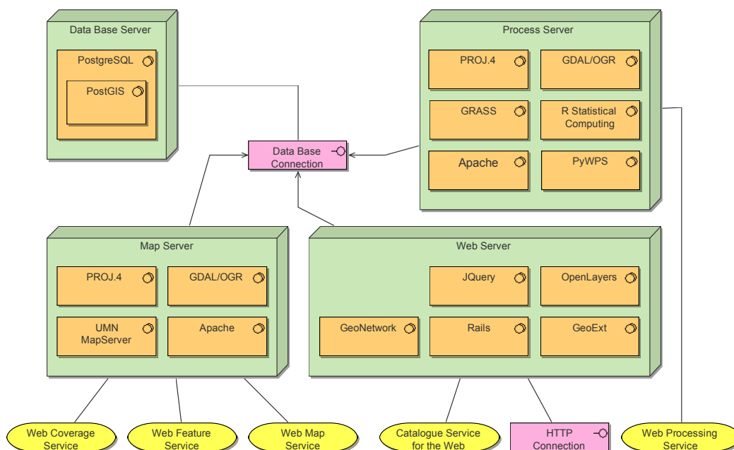
Figure 2: The Technological Architecture supporting iGUESS. In green are nodes, in orange software, in pink connections and yellow for services.
