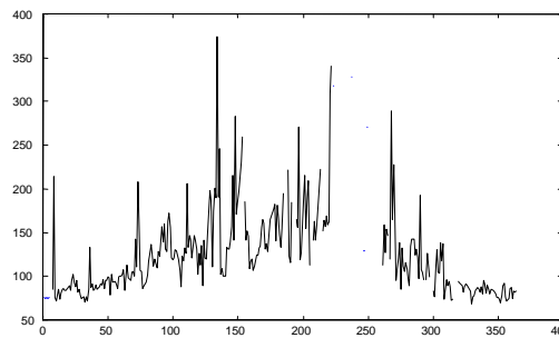
Figure 3b. Melilli, O 3 , Max per Day, 1999
