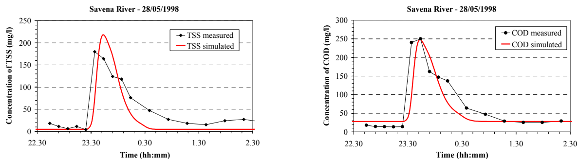
Comparison between simulated and measured TSS and COD in the Savena river (about 300 meters downstream the overflow) on May 28 th , 1998.
