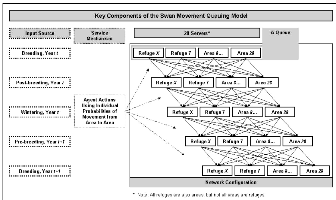
Figure 1. The D/DB/28 configuration of the queuing model.
