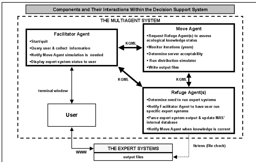
Figure 2. The decision support system consists of a multiagent system of 3-9 agents that interacts with three expert systems to implement the queuing model.
