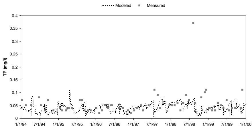
Figure 4. Observed and modeled TP for the calibration (1994-1997) and validation periods (1997-2000) at Silberhuetten water quality gauge station
