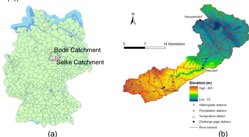
Figure 1. (a) Location of Selke catchment; (b) Map showing catchment elevation, stream network, precipitation monitoring stations, climate station, discharge gauge stations, and water quality sampling locations
