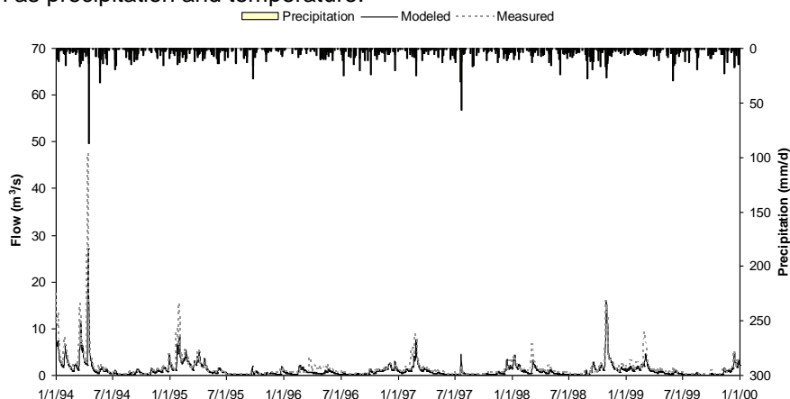
Figure 2. Observed and modeled stream flow for the calibration (1994-1997) and validation (1997-2000) periods at Silberhuetten discharge gauge station
