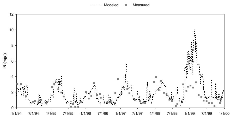
Figure 3. Observed and modeled IN for the calibration (1994-1997) and validation periods (1997-2000) at Silberhuetten water quality gauge station
