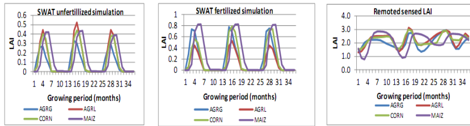
Figure 2. Leaf area index (LAI) values for a three year SWAT simulation period for a scenario with no fertilizer, with fertilizer, and corresponding remotely sensed LAI
