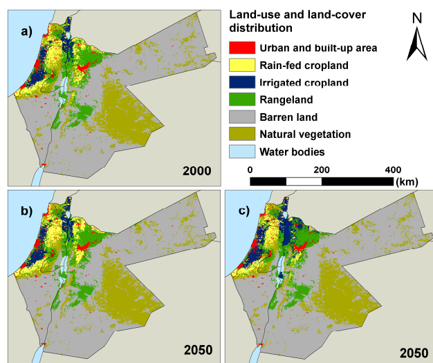
Figure 2. Land-use and land-cover distribution in a) the base year (2000) and the year 2050 for b) one example (ECv3.5-NoDemC) with constant demands and climate change, and c) NoCC-DemJRR.
