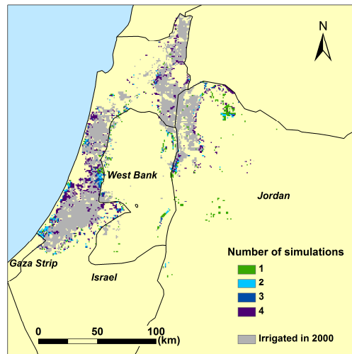
Figure 3. Number of simulations with climate change projecting a conversion to irrigated cropland through 2050.
