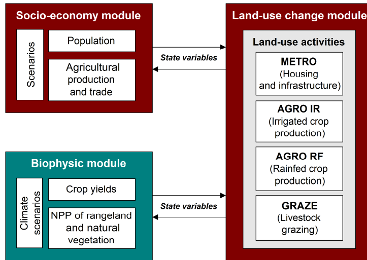
Figure 1 Schematic representation of the modeling framework LandSHIFT.
