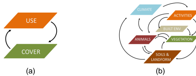
Figure 1. Two examples of conceptual land systems models. a) a simple 2-component model consisting of land use and land cover; b) a generalised land systems model.
