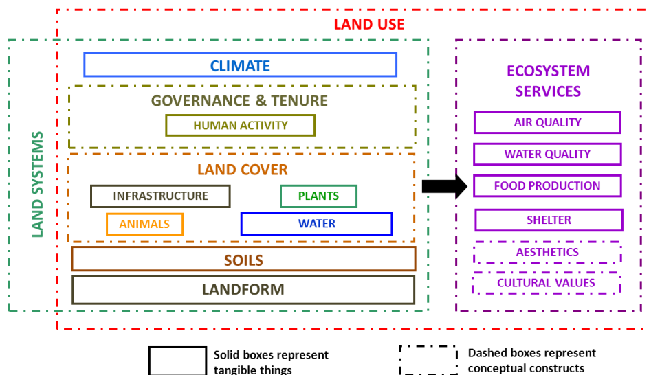
Figure 2. Conceptual approach to modelling the implications of land-use and land-cover change on ecosystem services.
