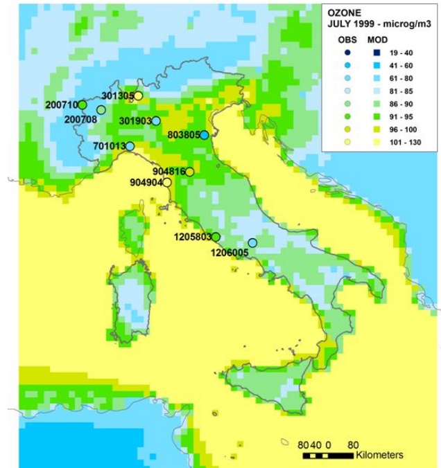
Figure 4. Comparison between observed (circles) and simulated data (AMS gridded output) for ozone hourly concentrations averaged over July 1999.
