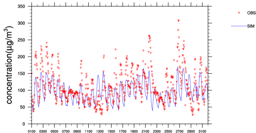
Figure 3. Ozone hourly measured values (red dots) and model results (blue line) at 301305-Varenna station, during July 1999.
