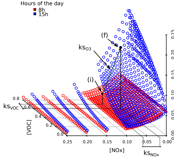
Figure 2: Subset of the LUT for two different hours, 8 and 15 hours of the day. The ozone and \text{NO}_x concentrations are in ppm and the VOC concentrations are in ppmC. Point (i) represents a possible initial point at 8 hours, and (f) represents the resulting ozone concentration (ppm) 7 hours later. The reaction coefficients K_{s\text{NO}_x} , K_{s\text{VOC}} and K_{s\text{O}_3} are calculated according to Eq. 1.
