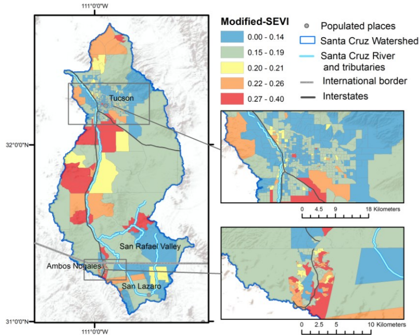
Figure 2. Map displaying a geometrical interval distribution of M-SEVI values in the Santa Cruz Watershed.
