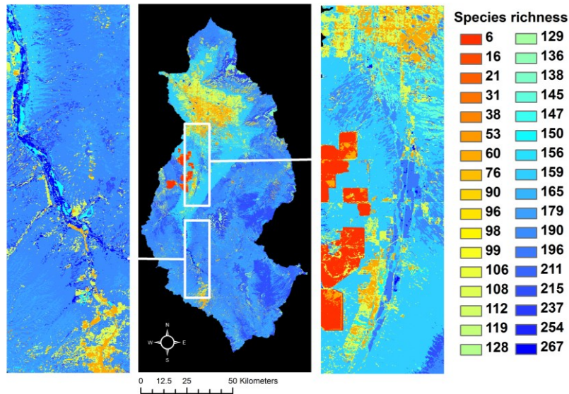
Figure 3. Species richness map of the Santa Cruz Watershed (center) including enlargements of the Santa Cruz River riparian corridor at the US/Mexico border (left) and Tucson metropolitan area (right).
