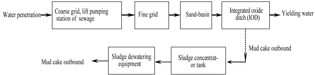
Figure.1 The diagram of XINDU wastewater treatment technology process flow
