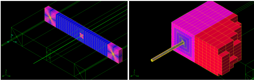
Figure 2. Detail of the mesh in this particular representation
