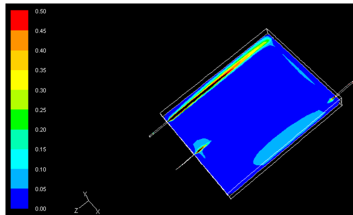
Figure 5. Detail of velocity magnitudes (in m/s) at mid-depth of the tank.
