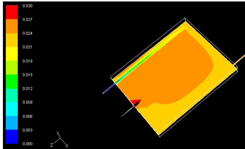
Figure 6. Illustration of the tracer mass fraction at mid-depth of the tank.
