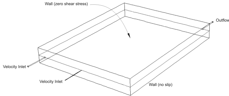
Figure 3. Boundary conditions defined for the rectangular tank
