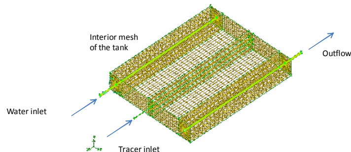
Figure 1. 3D geometry and mesh of the rectangular tank.
