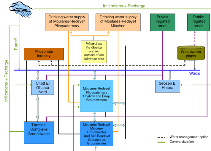
Figure 4. Conceptual scheme of the Gafsa mines influence area (Tunisia)
