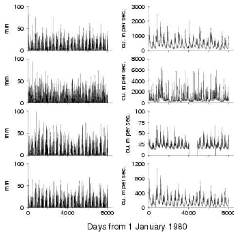
Figure 1. Daily rainfall and streamflow for (top to bottom) R. dos Bois, R. Ivaí, R. Preto and R. Meia Ponte
