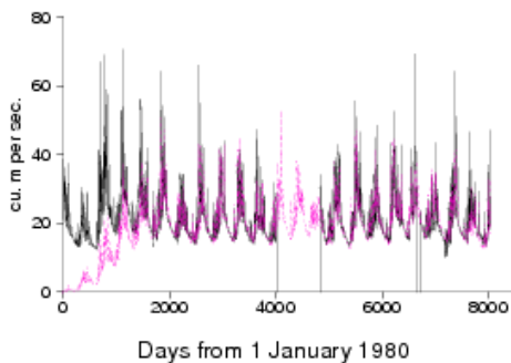
Figure 3. R. Preto: simulation-mode model-fit, 1980 to 2001
