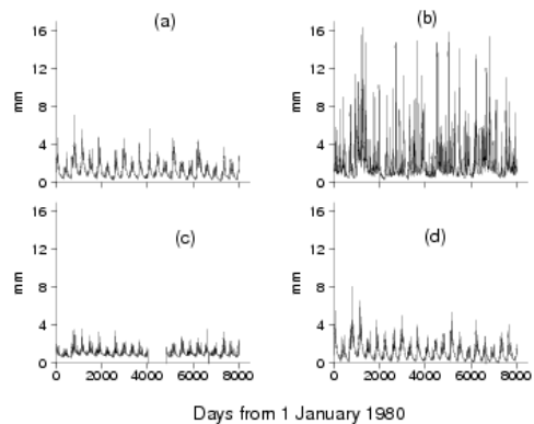
Figure 4. Daily runoff hydrographs 1980 to 2001 (a) R. dos Bois, (b) R. Ivaí, (c) R. Preto, (d) R. Meia Ponte
