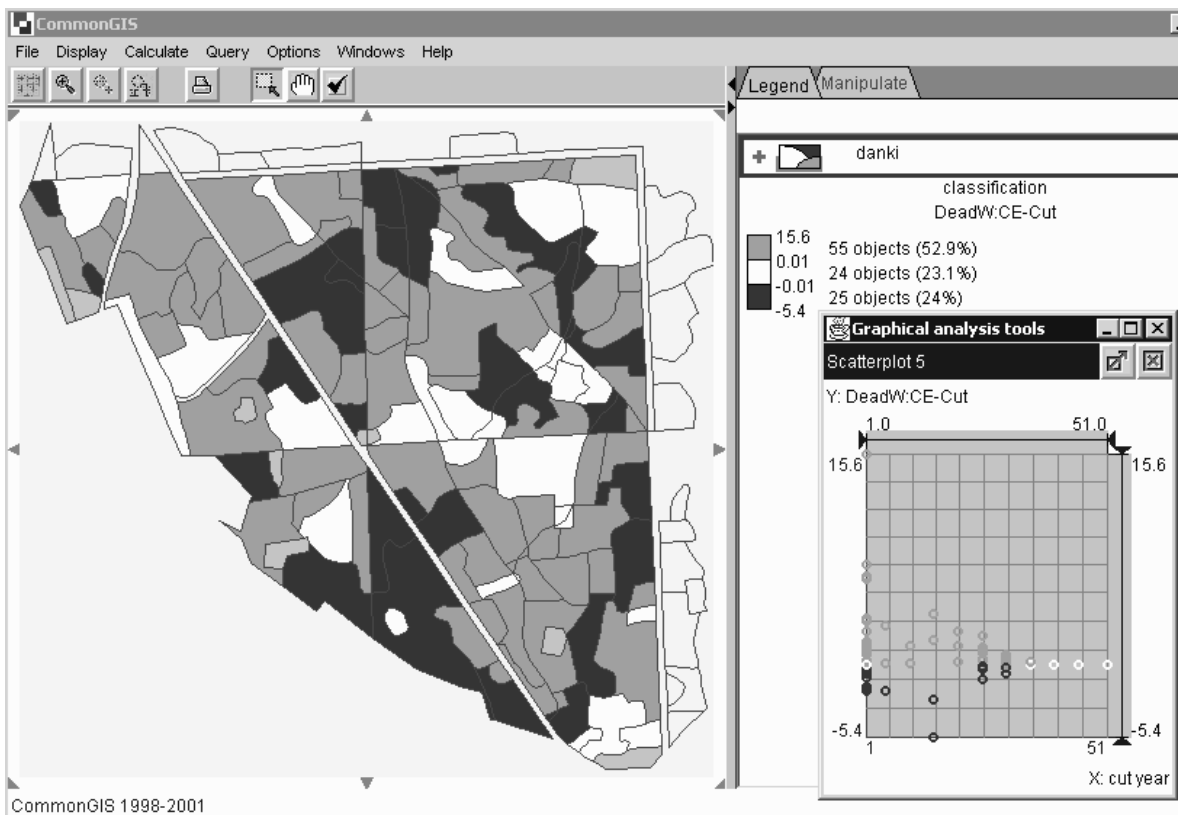
Figure 3. The relative advantage of ecologically oriented clear-cutting scenario in relation to Russian legal practice.
