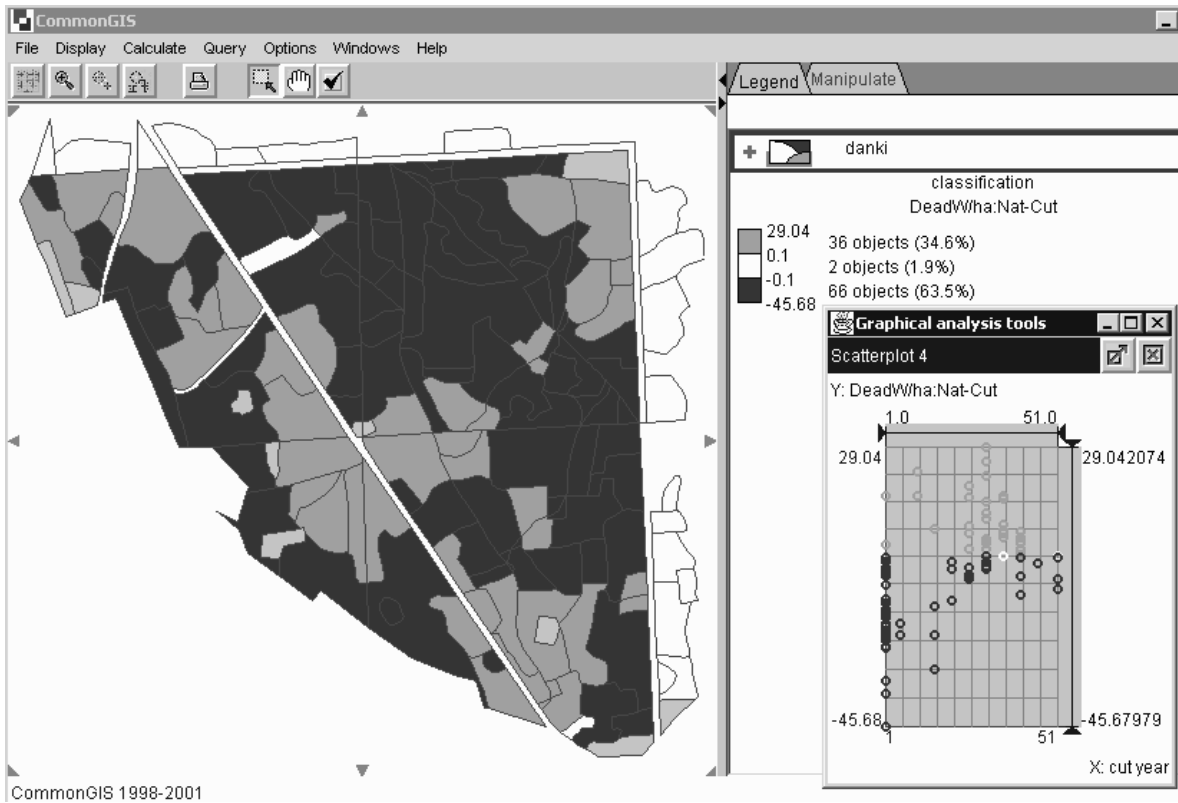
Figure 2. Difference of accumulated dead wood between natural development and cutting scenarios at the end of simulation.
