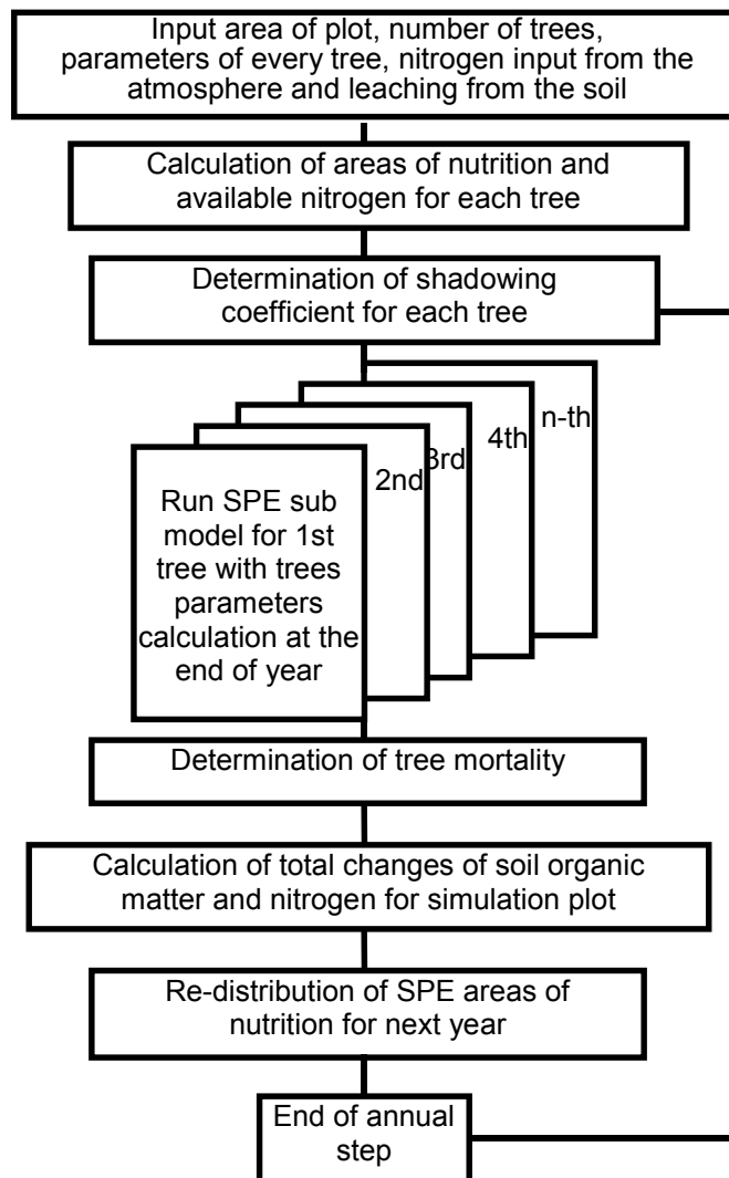
Figure 1. Flow-chart of year step of the EFIMOD model.
